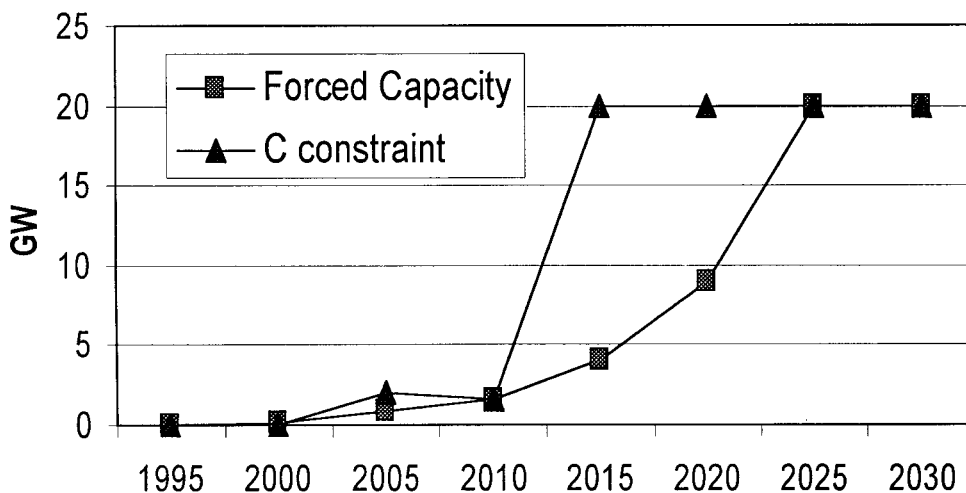
Figure 1. Capacity projections in the US-SW; scenarios of forced capacity and C constraints
