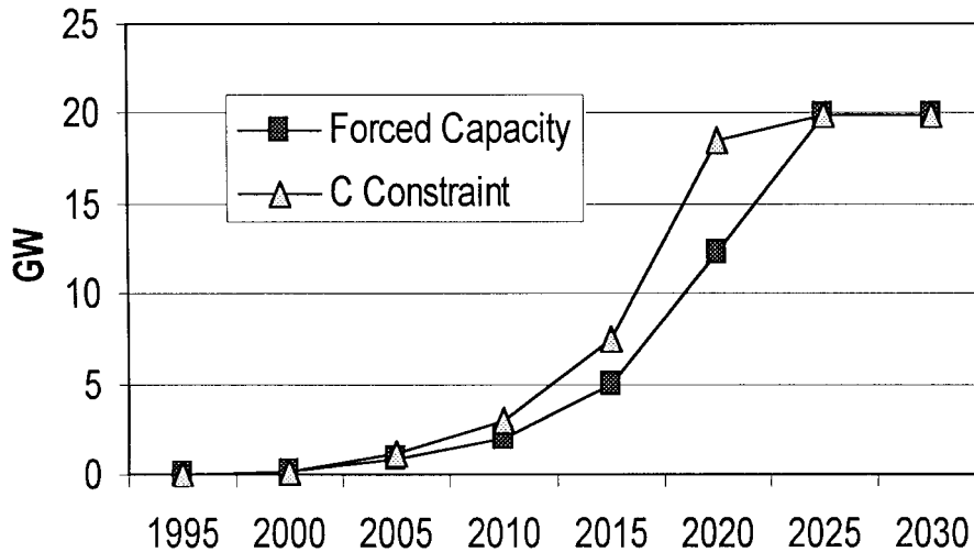
Figure 2. Capacity projections in the US-NE; scenarios of forced capacity and C constraints
